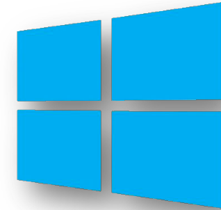
Directory Synchronization
